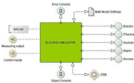
Fig. 3. General configuration of the simulator of an intelligent building.
