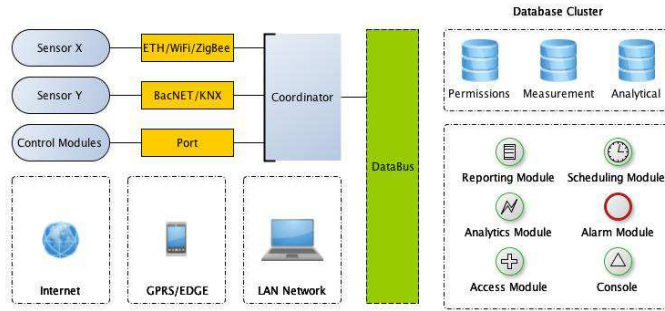
Fig. 1. Structure of the Network Object Monitor.
